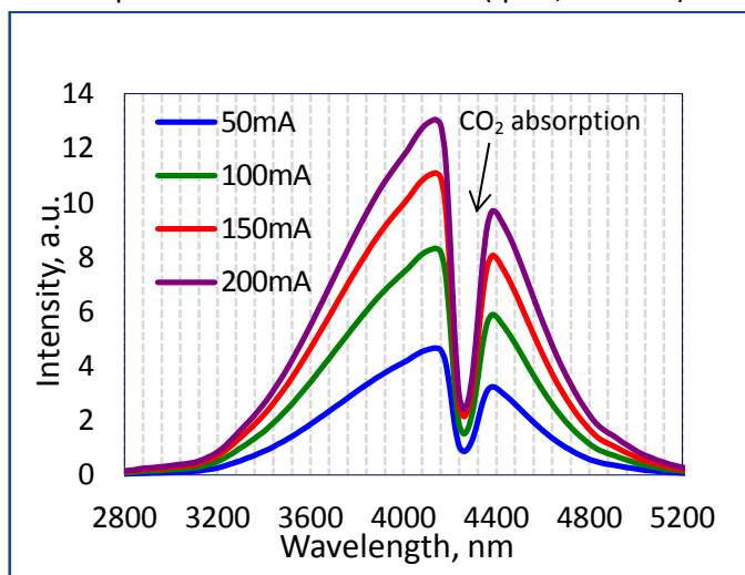
Spectra at different currents (qCW, T=300 K)
