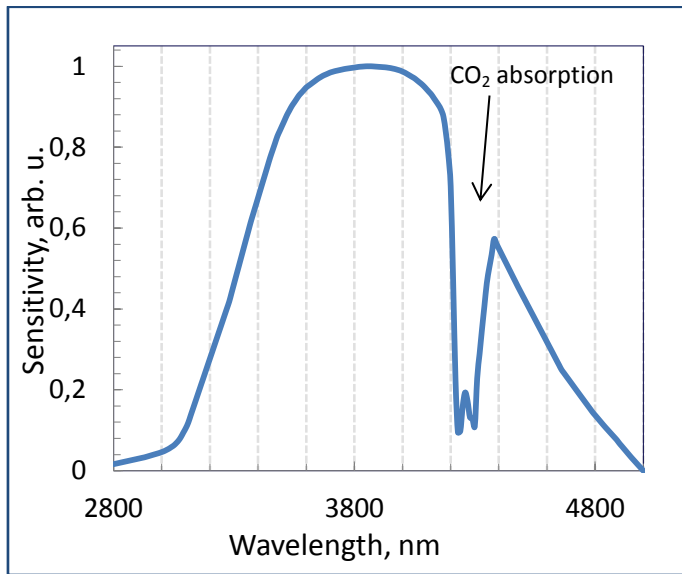
Spectral response (typical)
