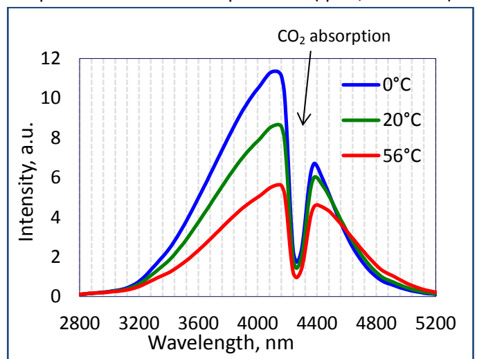
Spectra at different temperatures (qCW, I=150 mA)
