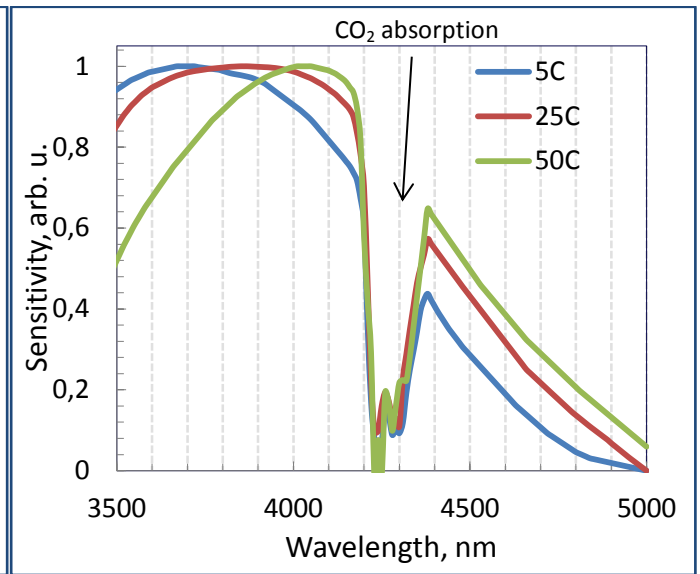
Temperature shift of spectral response
