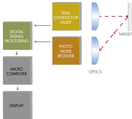
Schematic diagram of TOF principle.
